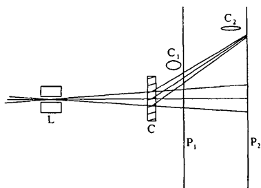
Fig. 1. Bragg's interpretation of the focusing of the diffracted spots observed by von Laue, Friedrich and Knipping which led to the formulation of Bragg's law: n\lambda = 2d \sin \theta . L, Lead screen; C, crystal; P_1P_2 , positions of photographic plate; C_1C_2 , cross sections of pencil of rays at P_1P_2 . [From Proc. Cambridge Philos. Soc. (1913), 17(1), 43.]
